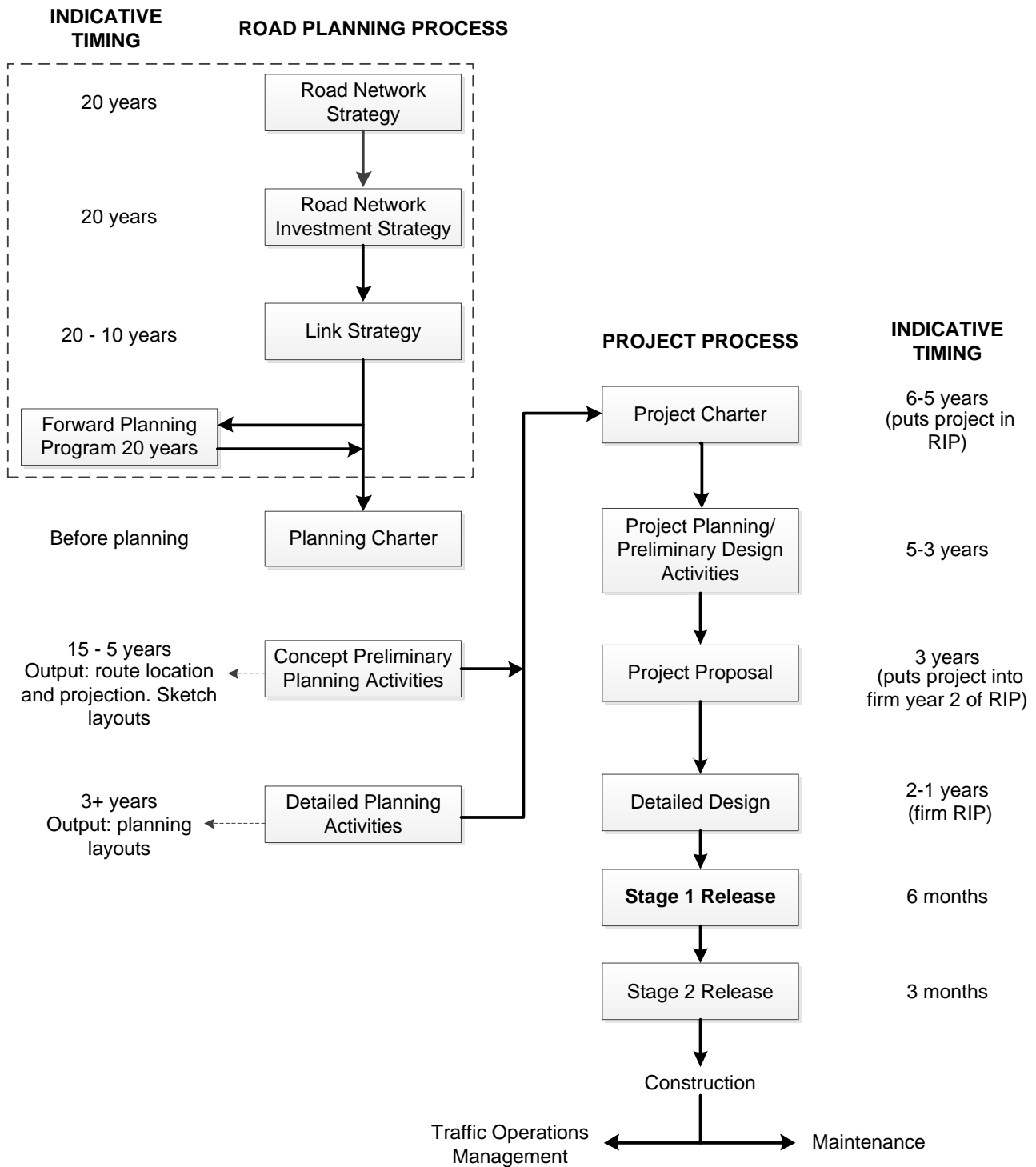
Figure 5.1: Typical road planning and design process
